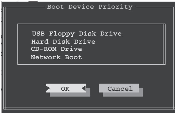
Figure 18. Boot Device Priority Submenu
